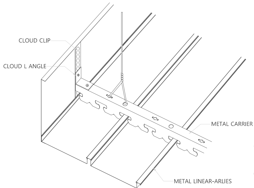
ARLIES METAL LINEAR CLOUD TRIM DETAIL
